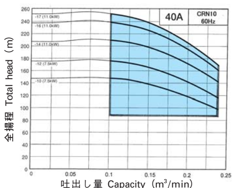
●選定図表(Selection chart) 回転速度 3,600min -1 (2極)
